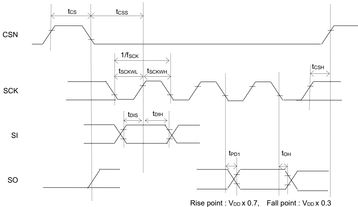
Figure 4 Input / Output and Setup / Hold timing
