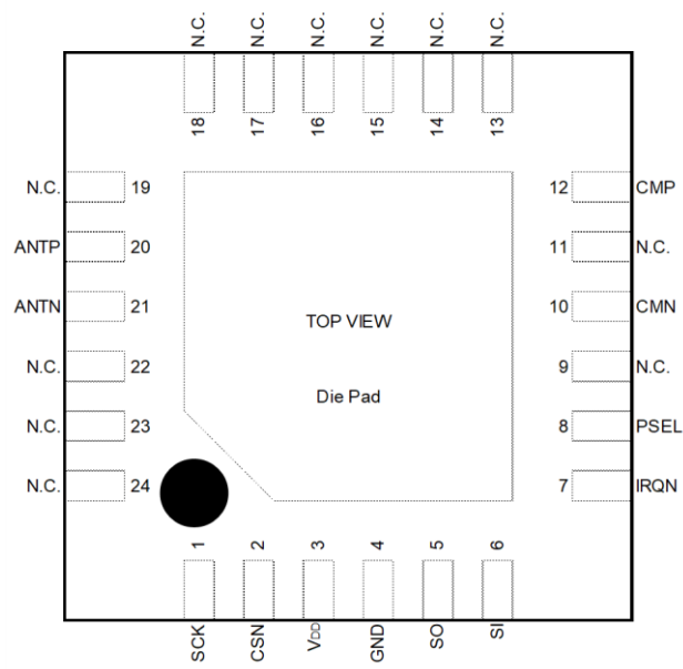
Figure 3 24pin WQFN
