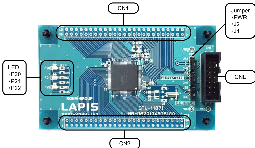
Fig. 1 ML62Q1749 Reference Board Outline Diagram
