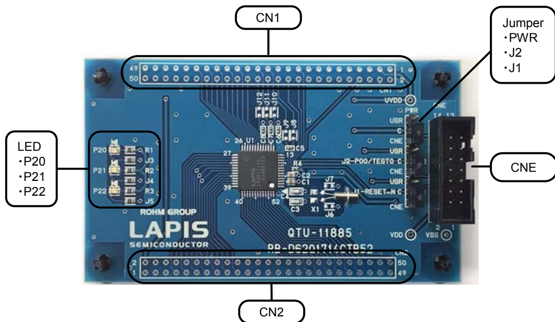
Fig. 1 ML62Q1714C Reference Board Outline Diagram
