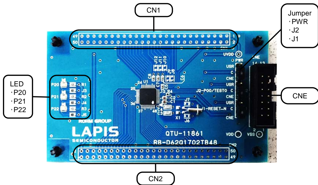
Fig. 1 ML62Q1702 Reference Board Outline Diagram
