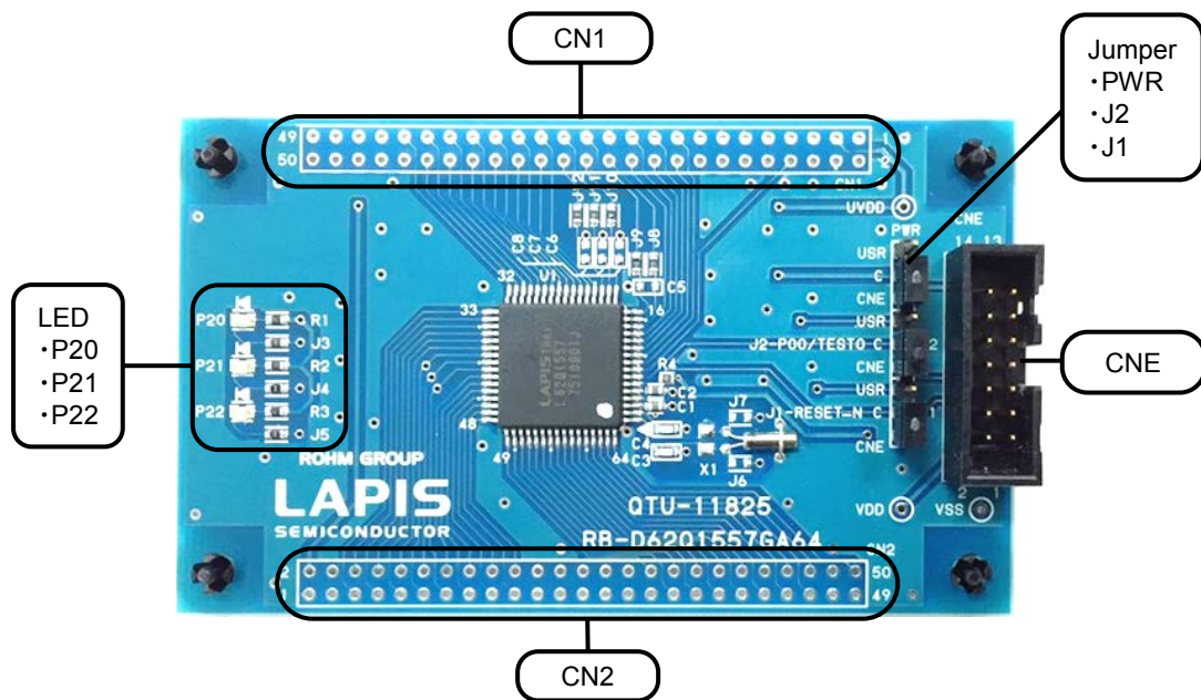
Fig. 1 ML62Q1557 Reference Board Outline Diagram
