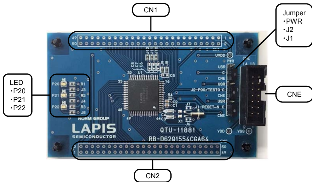
Fig. 1 ML62Q1554C Reference Board Outline Diagram
