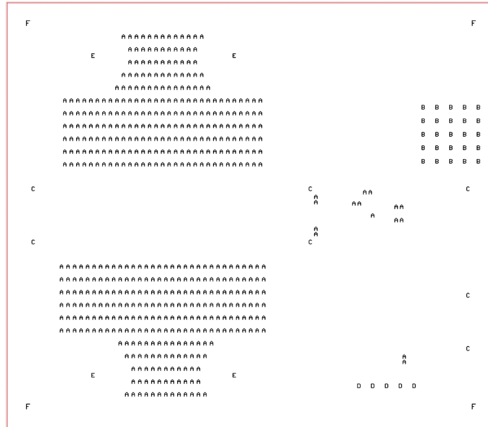
Drill Drawing(Top View)
