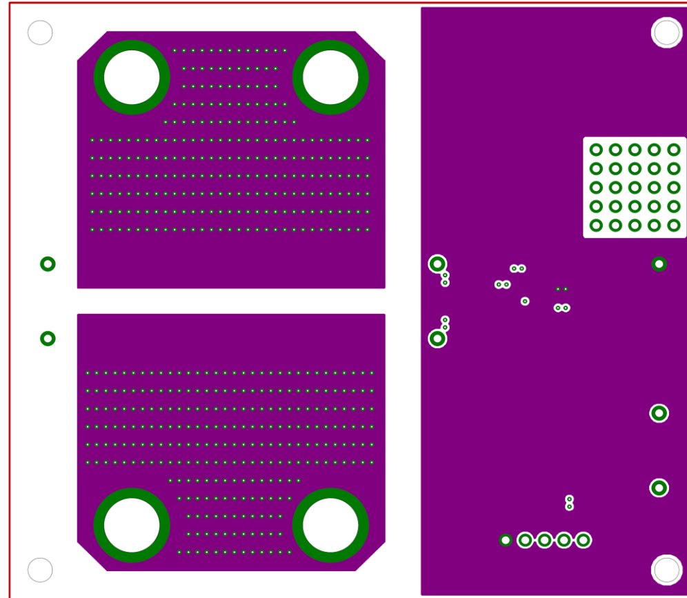
Midlayer2(Top View)
