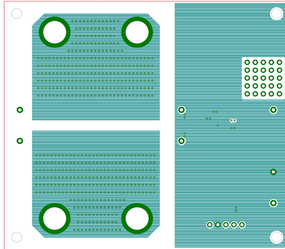
Midlayer1(Top View)
