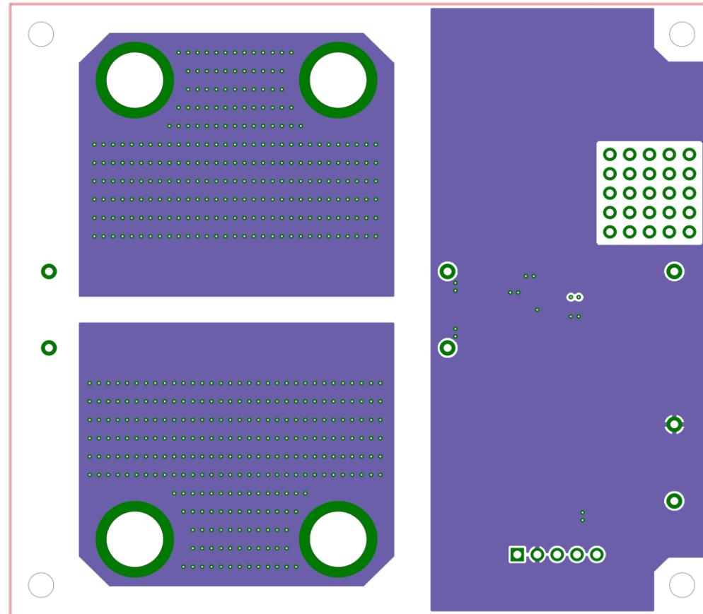
Bottom Layer(Top View)
