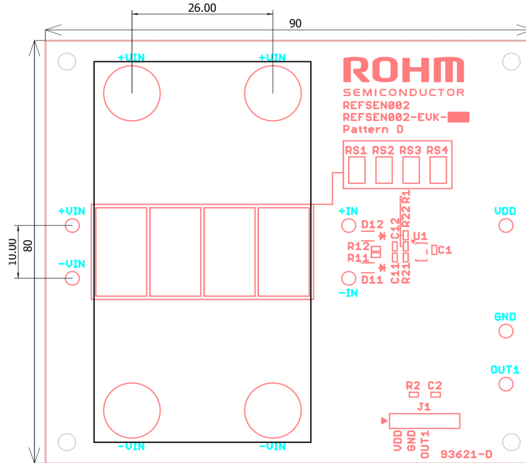
Top Silkscreen Overlay (Top View)
