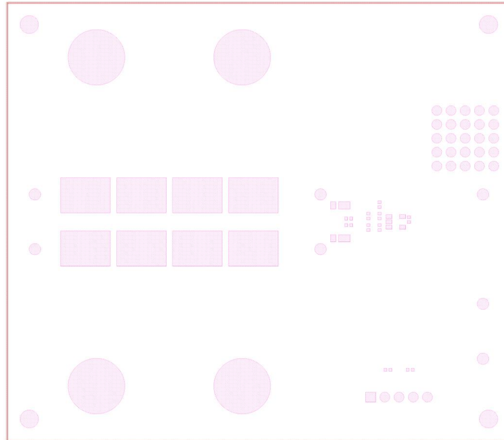
Top Solder Mask(Top View)
