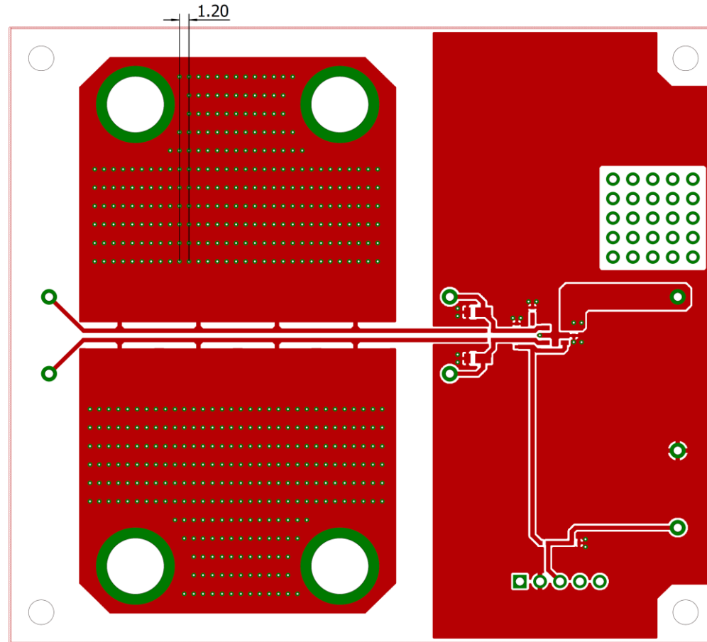
Top Layer(Top View)
