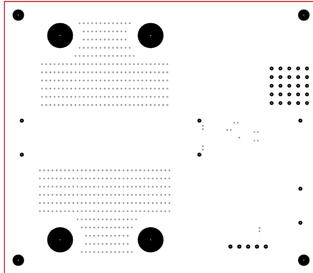
Drill Guide(Top View)
