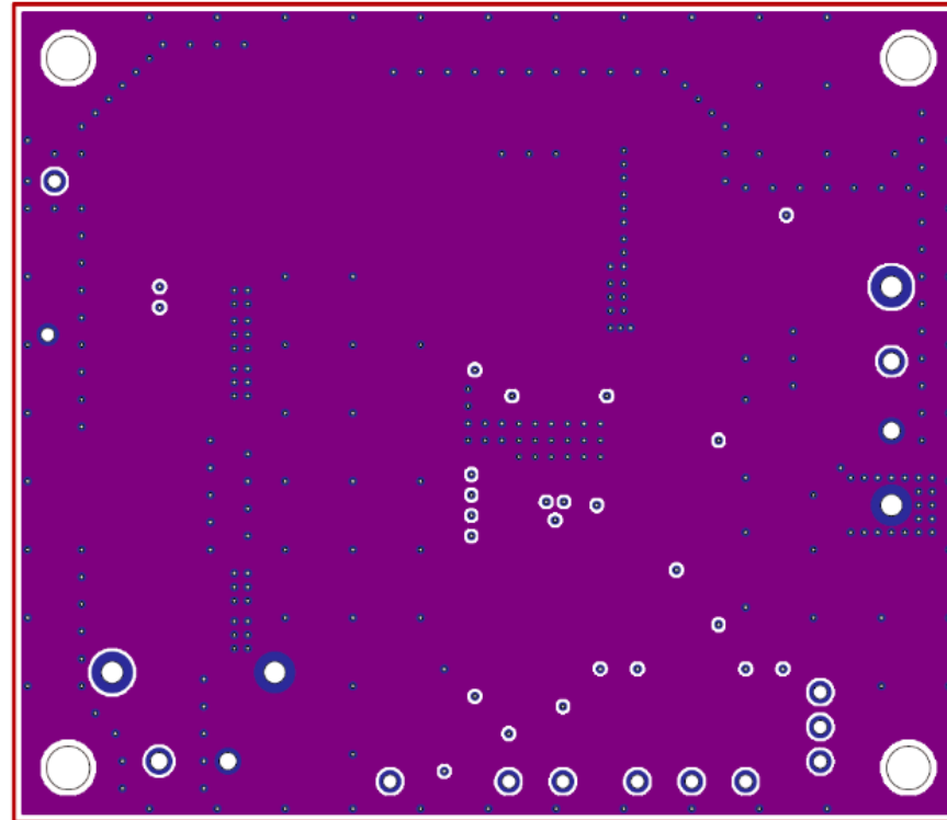
3rd layer layout(Top view)
