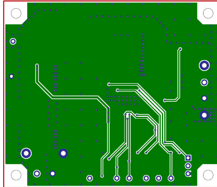
Bottom layer layout(Top view)
