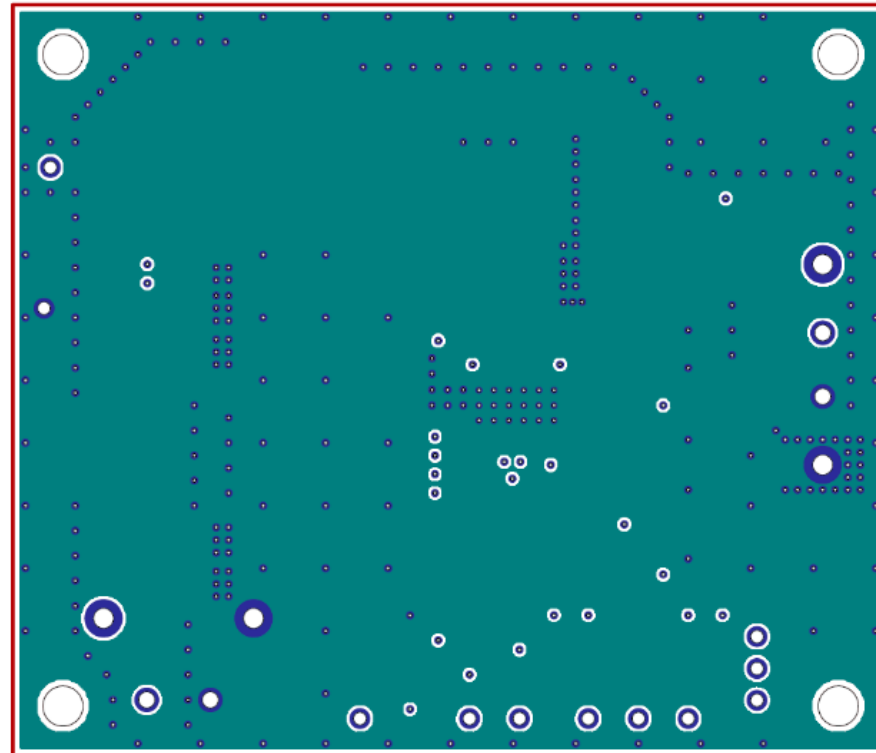
2nd layer layout(Top view)
