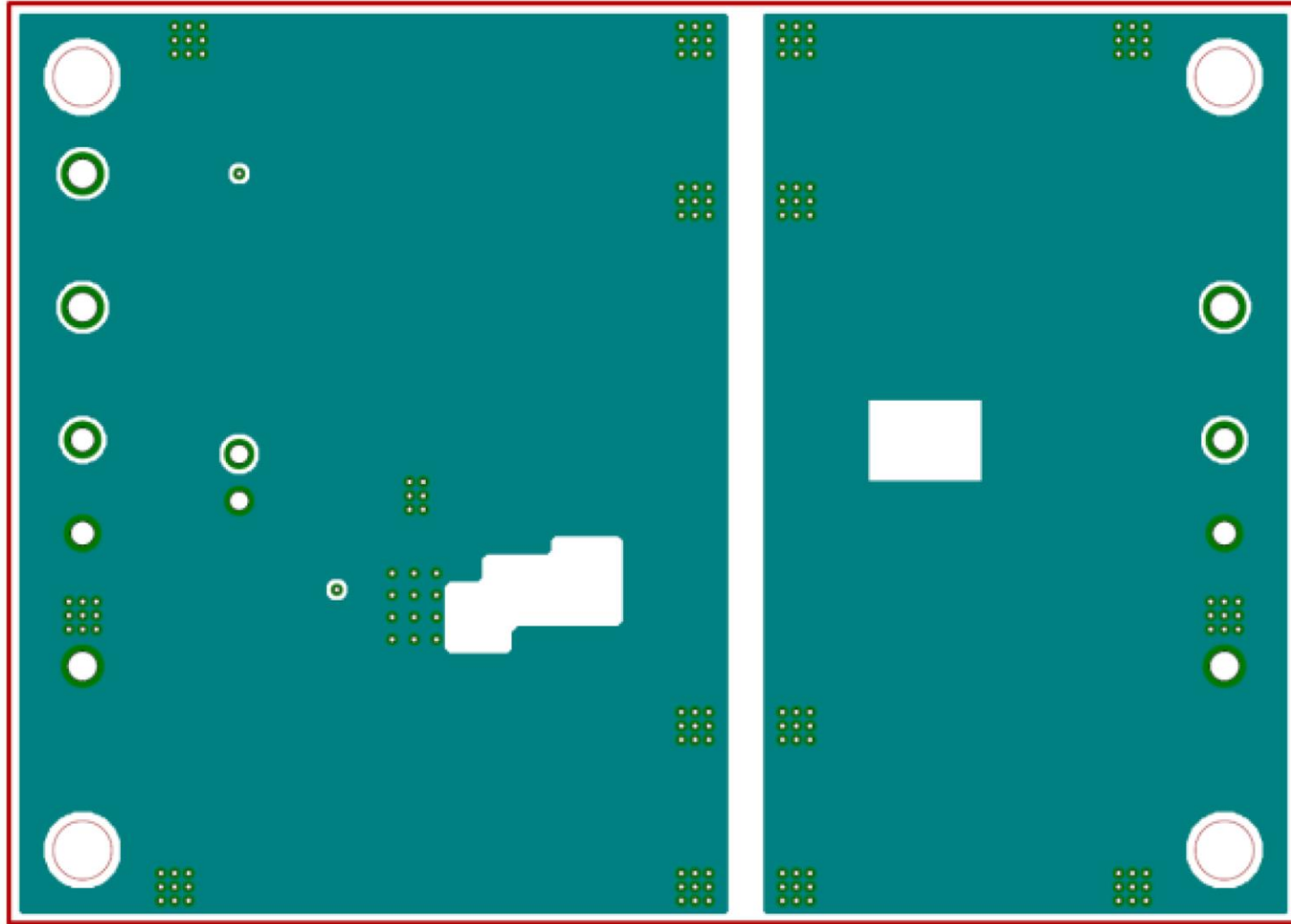
Middle Layer1 Layout
