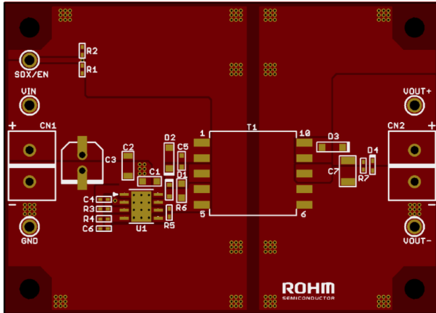
Top Silk Screen Layout
