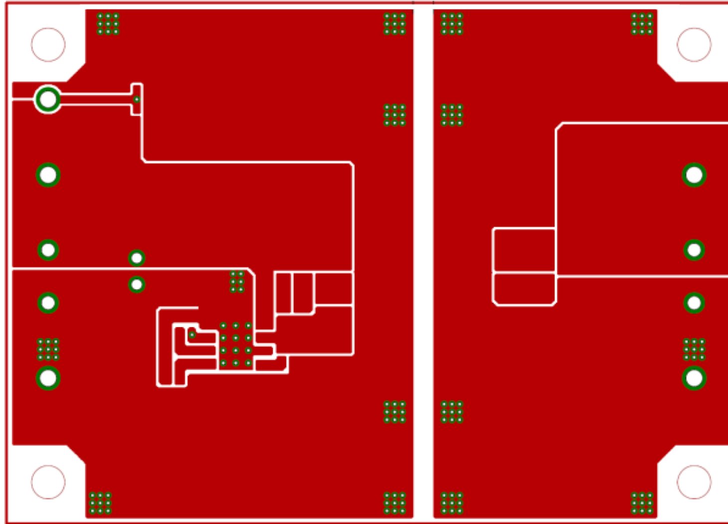
Top Side Layout
