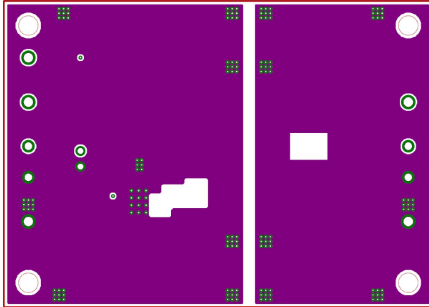
Middle Layer2 Layout
