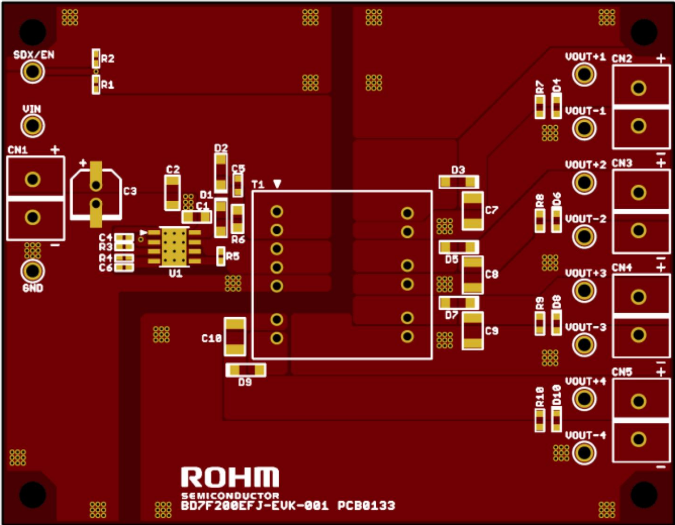
Top Silk Screen and Layout
