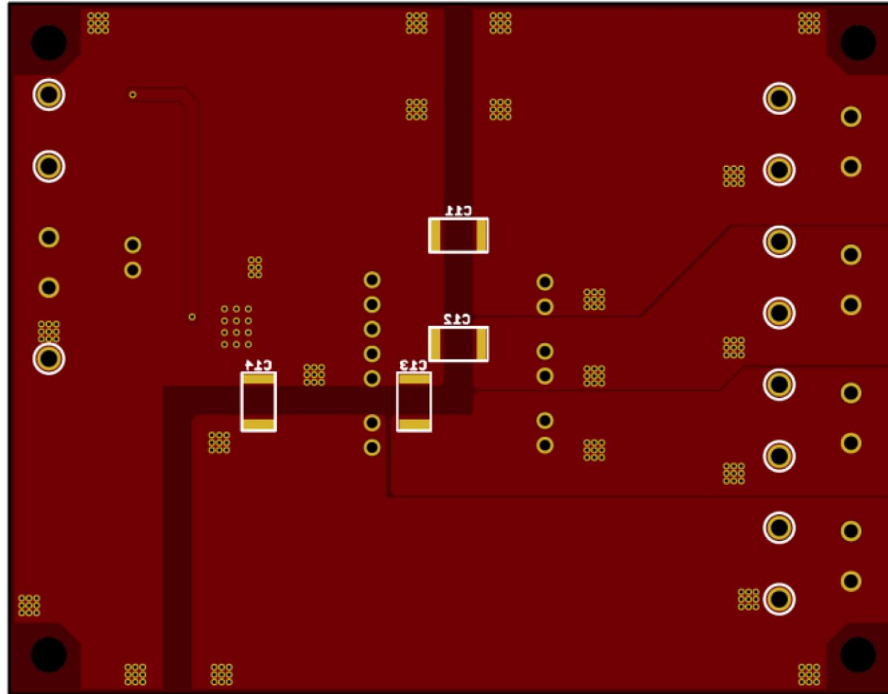
Bottom Silk Screen and Layout
