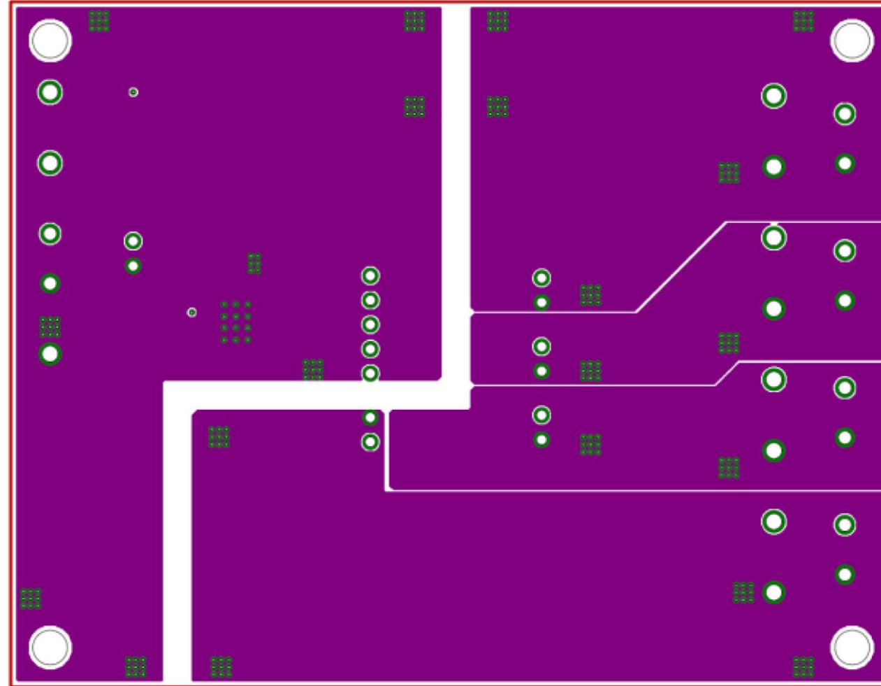
Middle Layer2 Layout
