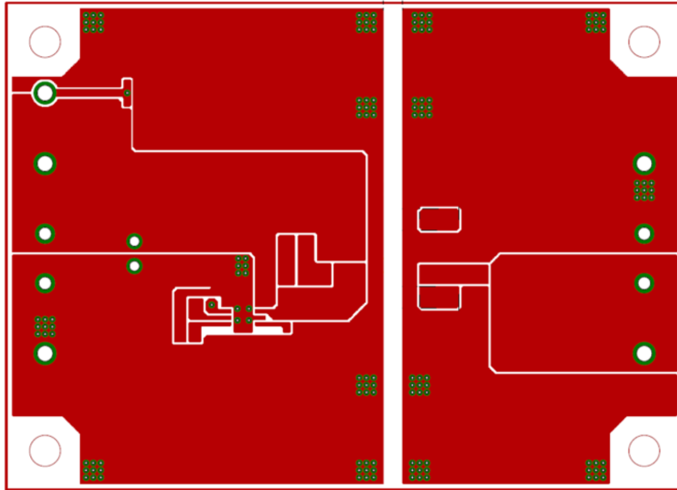
Top Side Layout
