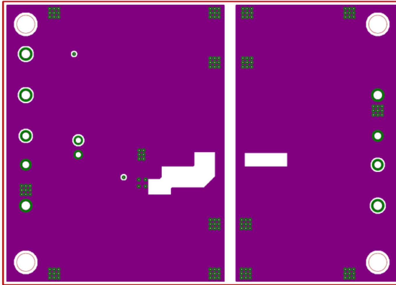
Middle Layer2 Layout
