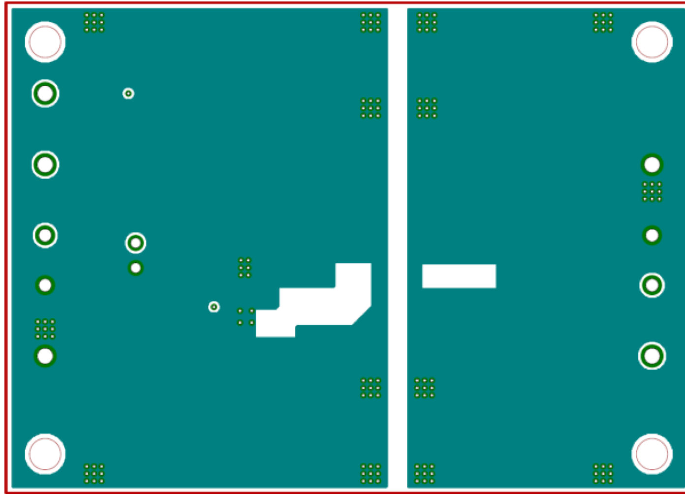
Middle Layer1 Layout
