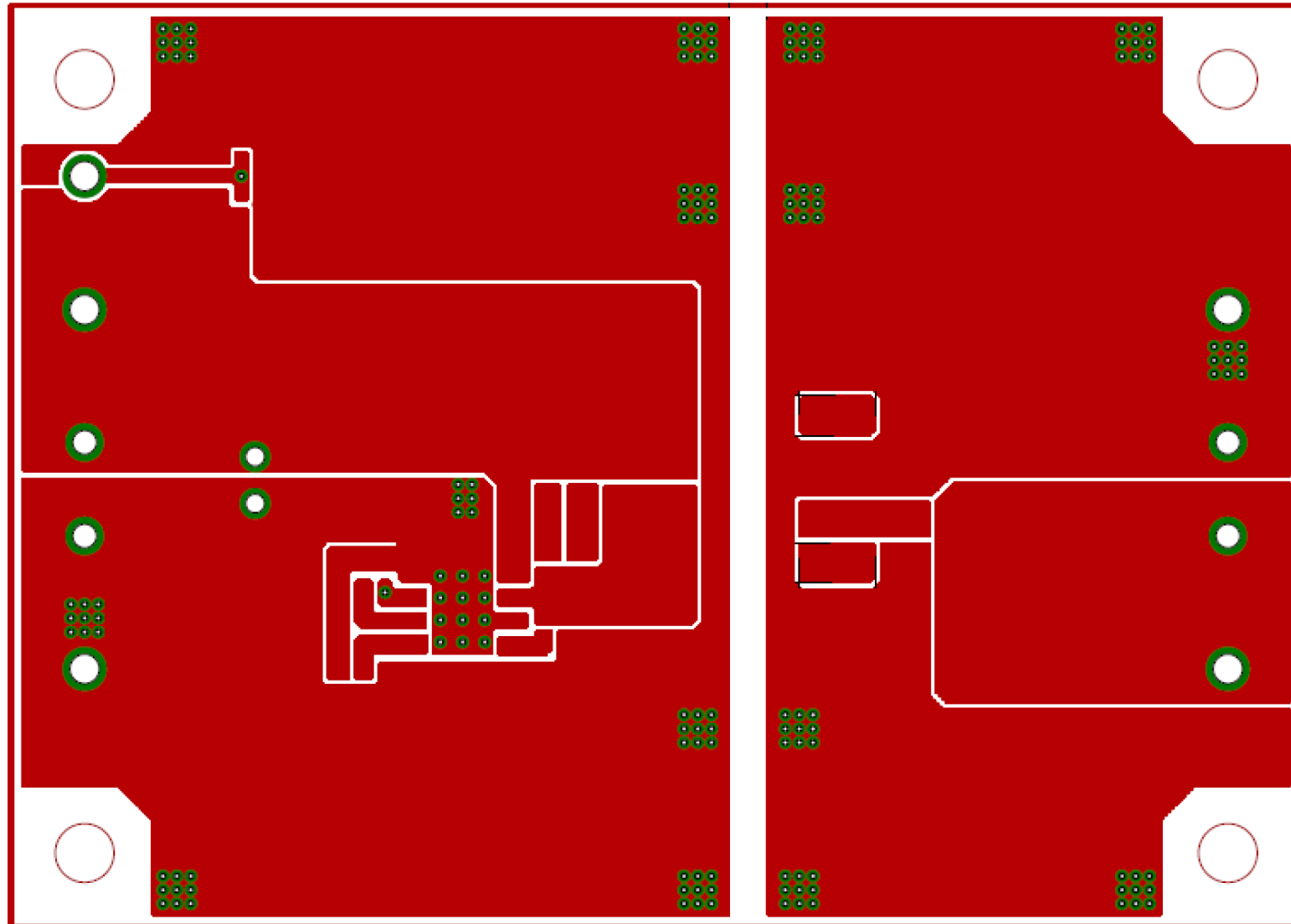
Top Side Layout
