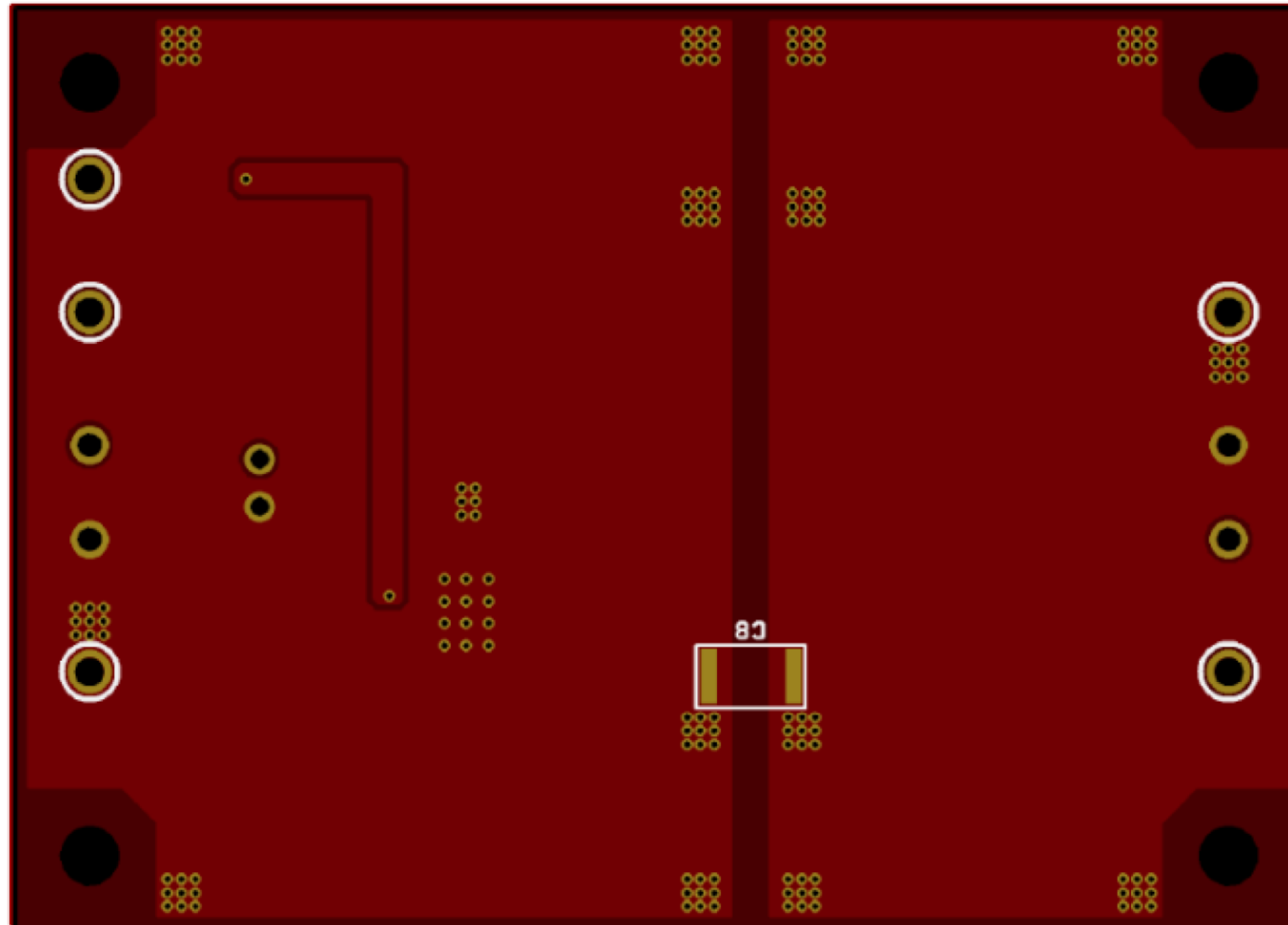
Bottom Silk Screen and Layout
