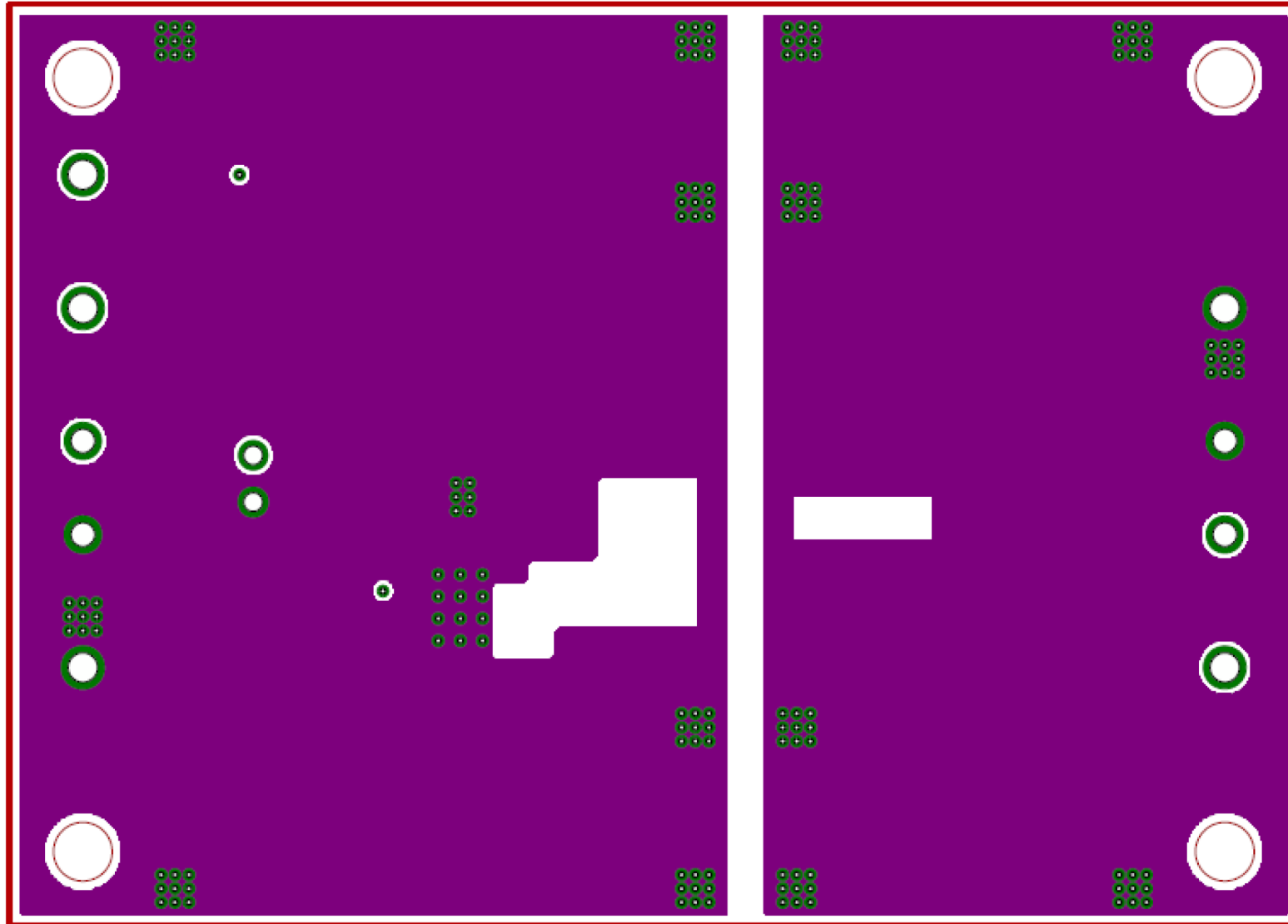
Middle Layer2 Layout
