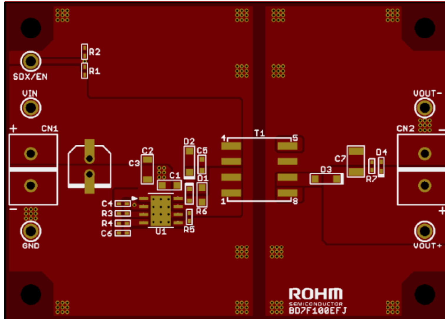
Top Silk Screen and Layout
