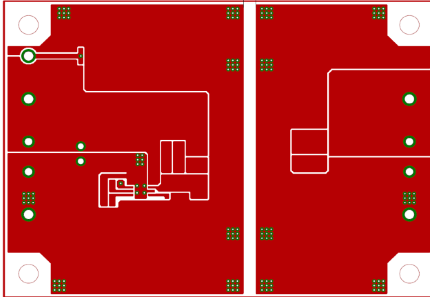
Top Side Layout
