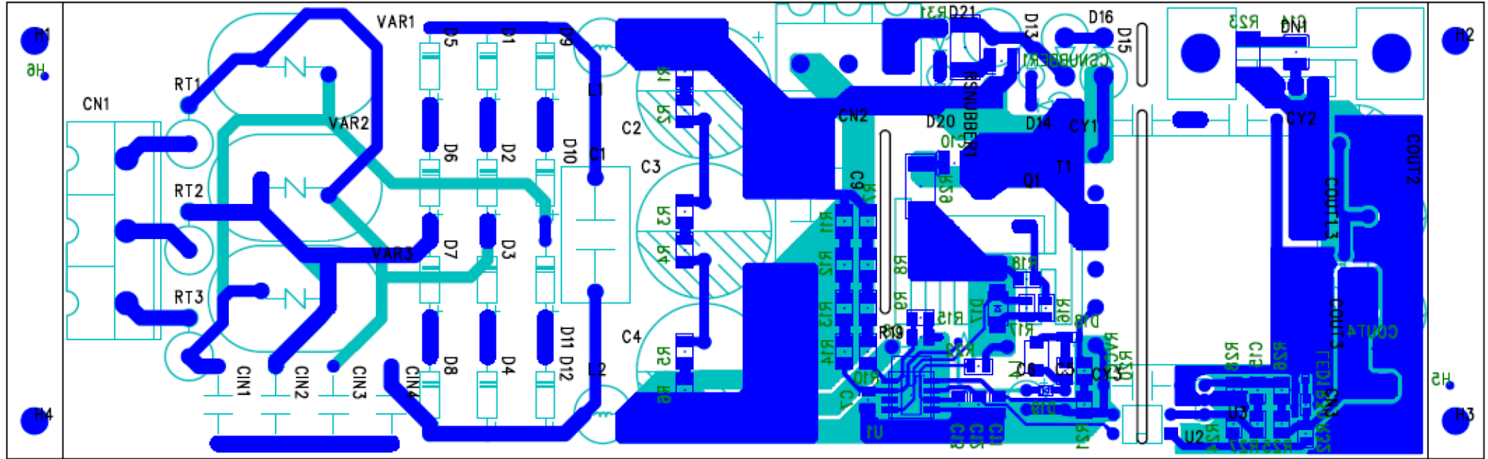
Proposed PCB Layout(Top view)
