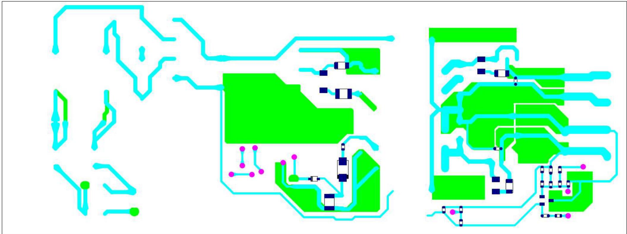
Bottom Layout (Top view)
