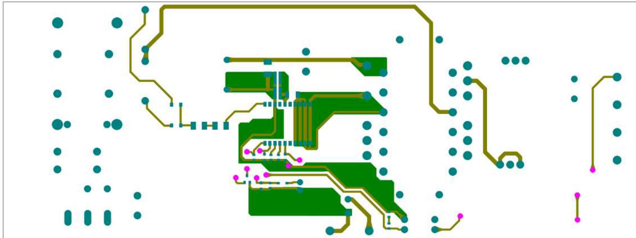
TOP Layout (Top view)
