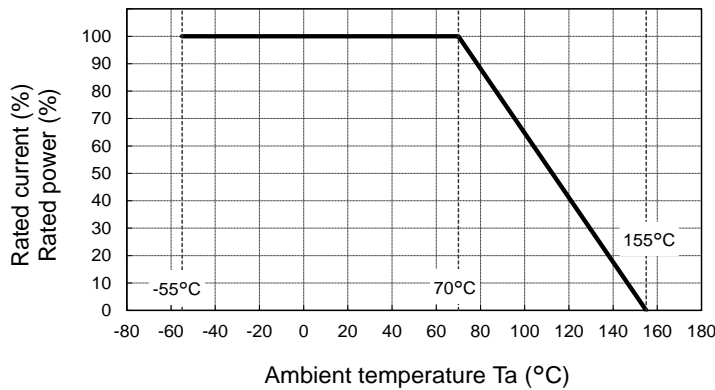
Fig.2< Terminal temperature>
