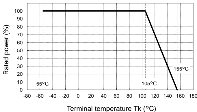
Fig.3< Terminal temperature>
