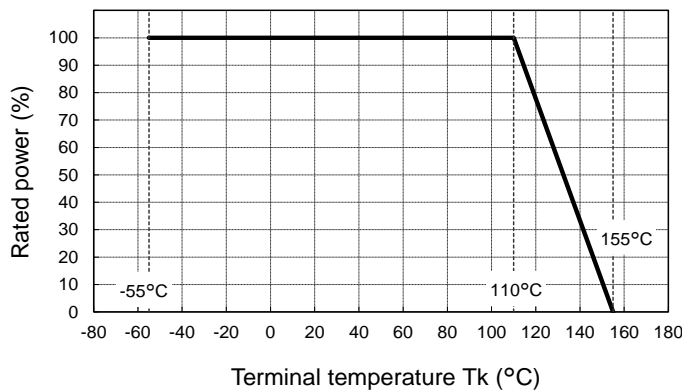
Fig.3< Terminal temperature>
