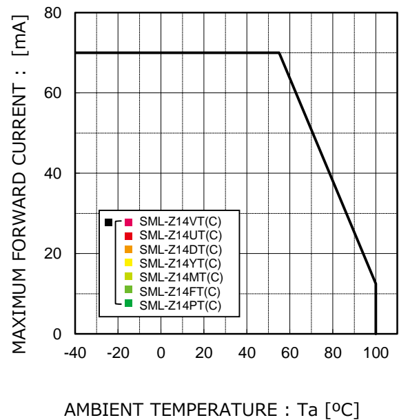
Fig.4 Derating
