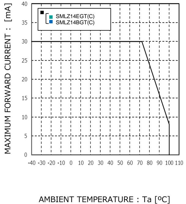
Fig.4 Derating
