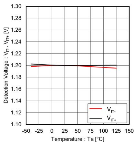
Figure 4. Detection Voltage vs Temperature ( V_{DD} = 3\text{ V} )
