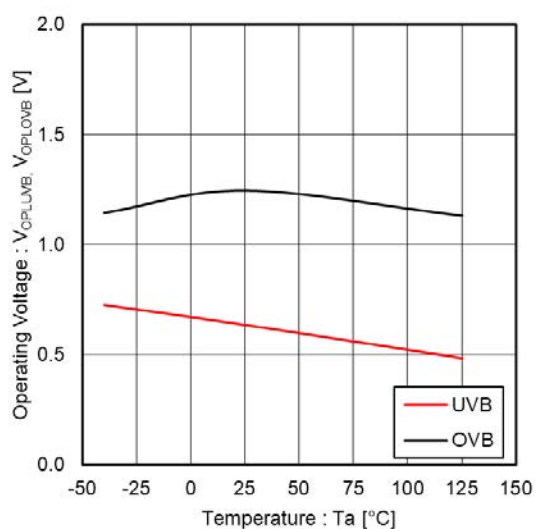
Figure 7. Operating Voltage vs Temperature
