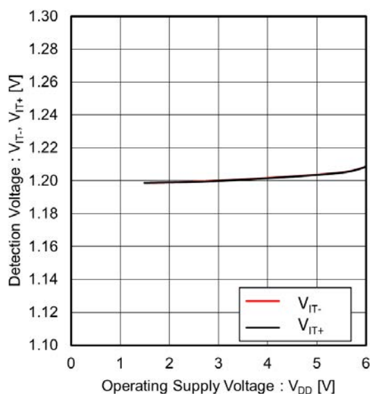
Figure 3. Detection Voltage vs Operating Supply Voltage ( T_a = 25\text{ °C} )
