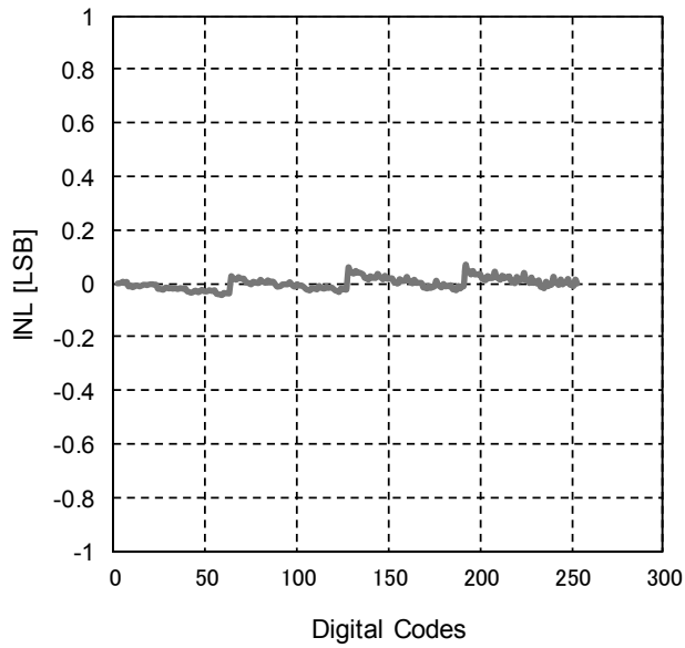
Fig.45 VCOM INL
