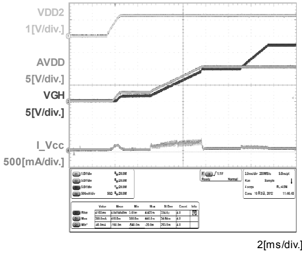
Fig.27 VGH Start-up Sequence
