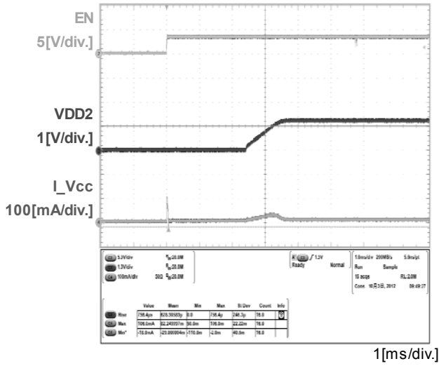
Fig.14 VDD2 Start-up Sequence
