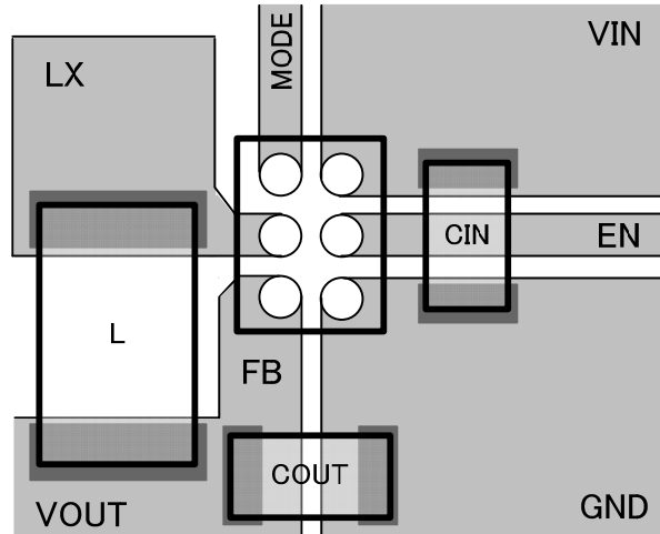
Figure 16. PCB layout
