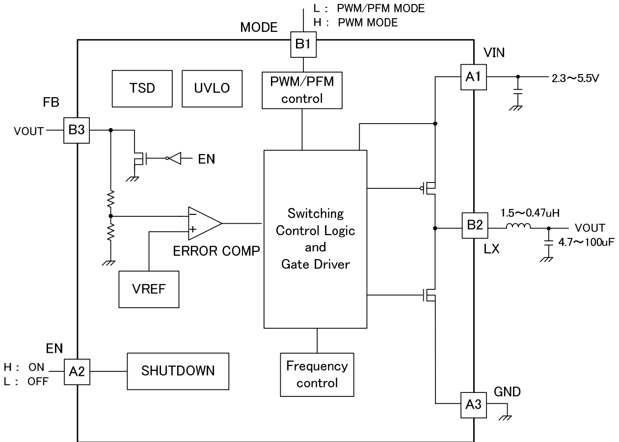
Figure 3. Block Diagram(s)
