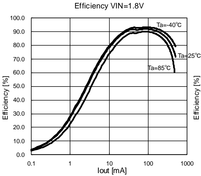
Figure 10. Efficiency PWM VIN=1.8V
