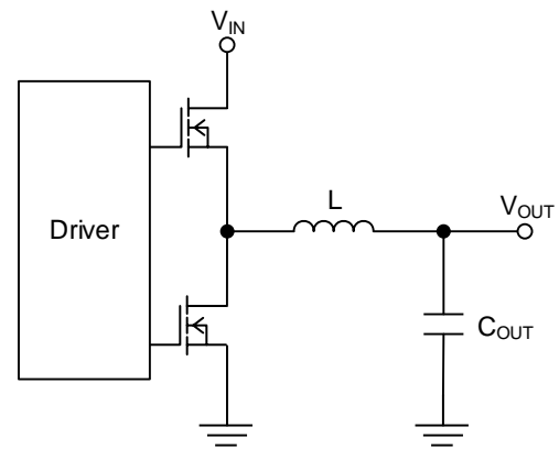
Figure 52. Output LC Filter Circuit
