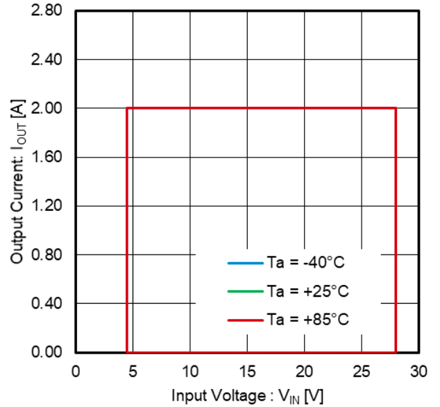
Figure 18. Output Current vs Input Voltage Operating Range: T_j < 150\text{ }^\circ\text{C} ( V_{OUT} \leq 1.8\text{ V} )
