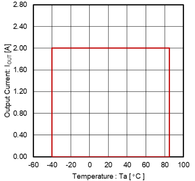
Figure 26. Output Current vs Temperature (Note 1) Operating Range: T_j < 150\text{ }^\circ\text{C} ( V_{IN} = 5\text{ V}, 12\text{ V}, V_{OUT} = 1.2\text{ V} )
