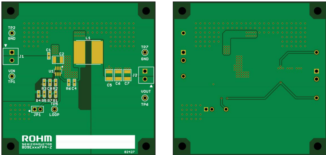
Figure 56. Example of PCB Layout (Silkscreen Overlay)
