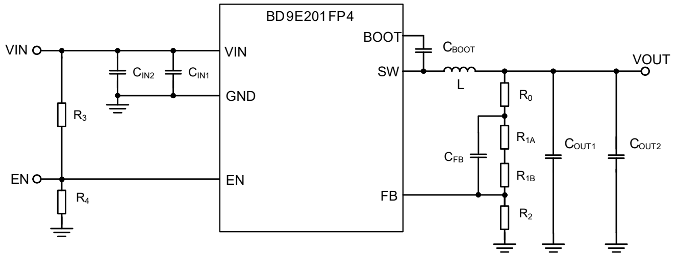
Figure 46. Application Circuit
