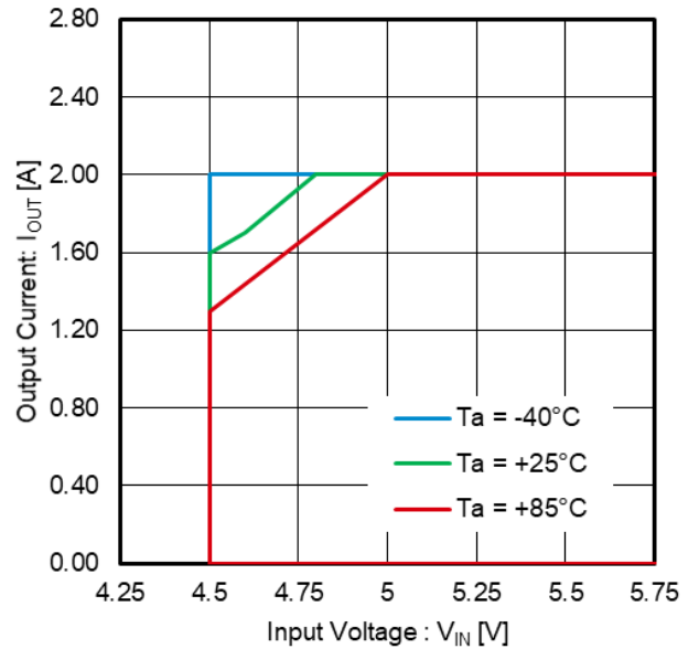
Figure 20. Output Current vs Input Voltage Operating Range: T_j < 150\text{ }^\circ\text{C} ( V_{OUT} = 3.3\text{ V} )
