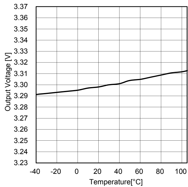
Figure 21. Output Voltage vs. Temperature (BD99010EFV-M: VOUT.3.3V)
