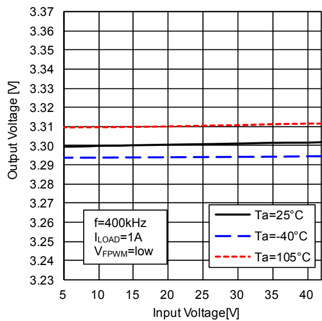
Figure 18. Line Regulation 1 (BD99010EFV-M: VOUT.3.3V)
