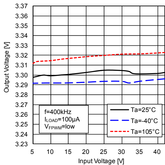
Figure 19. Line Regulation 2 (BD99010EFV-M: VOUT.3.3V)
