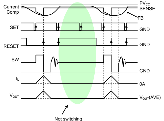
Figure 8. SLLM TM switching timing chart
