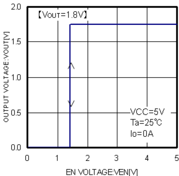
Figure 12. V_{OUT} VS V_{EN}
