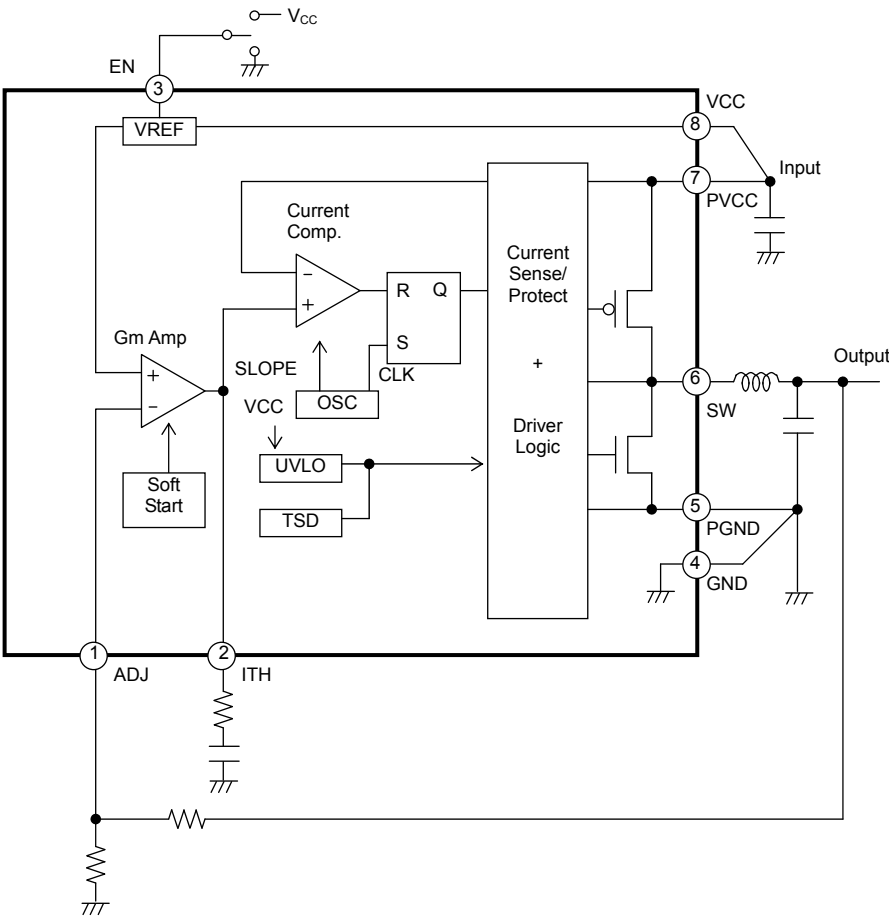
Figure 3. Block Diagram
