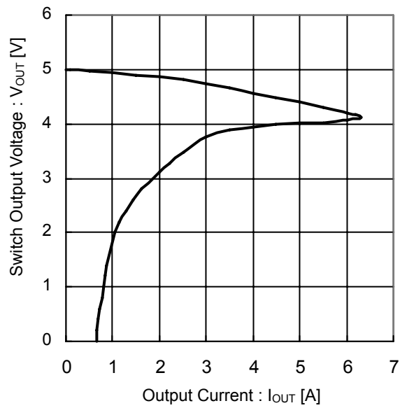
Figure 27. Switch Output Voltage vs Output Current (V IN =5.0V)
