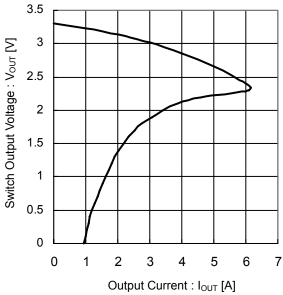
Figure 26. Switch Output Voltage vs Output Current (V IN =3.3V)
