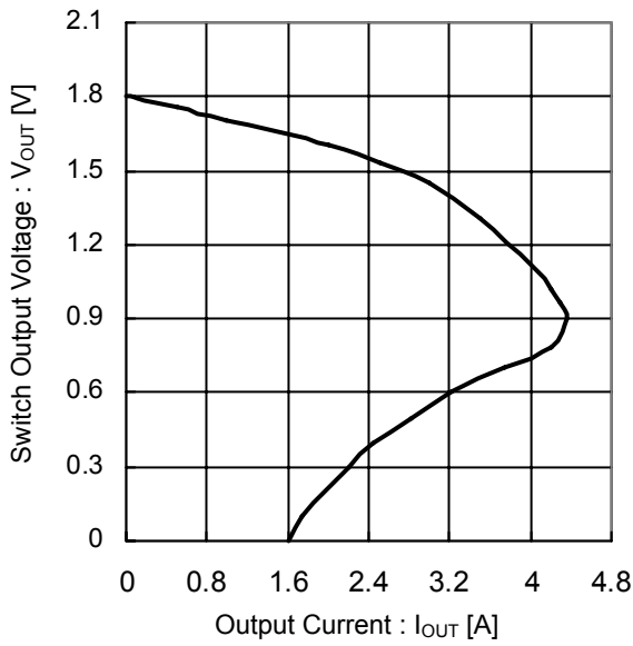
Figure 24. Switch Output Voltage vs Output Current ( V_{IN}=1.8V )
