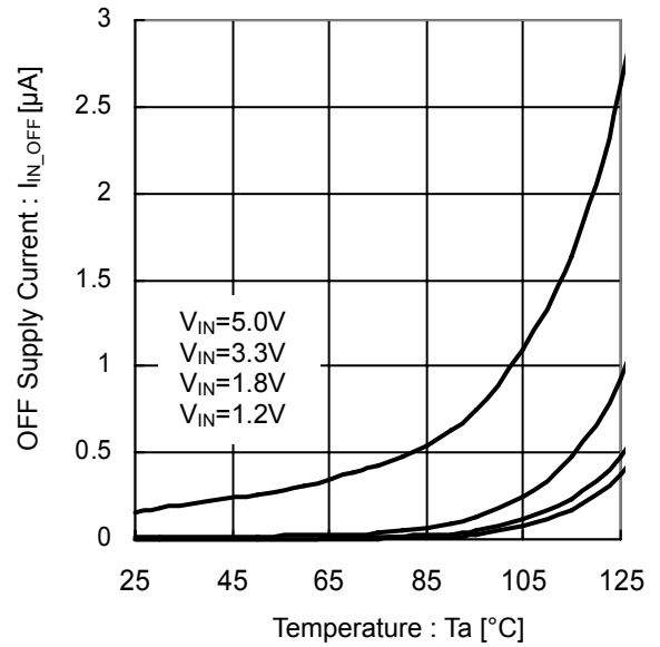
Figure 11. OFF Supply Current vs Temperature ( V_{EN}=0V )
