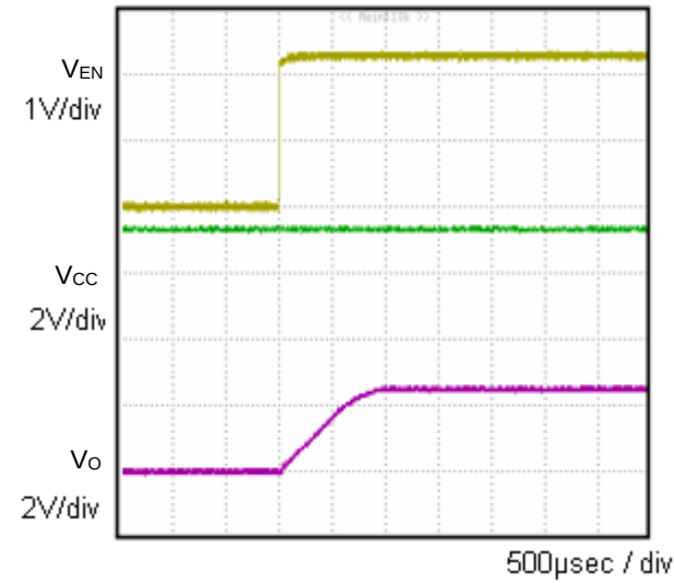
Fig.7 Input sequence 2 Co=1µF
