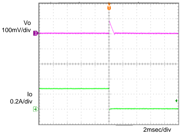
Figure 6. Transient Response (0.3→0A) Co=1\mu F , T_a=-40^\circ C
