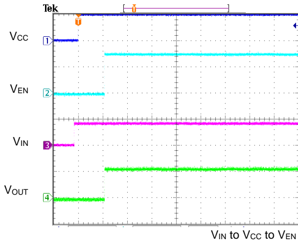
Figure 17. Input Sequence
