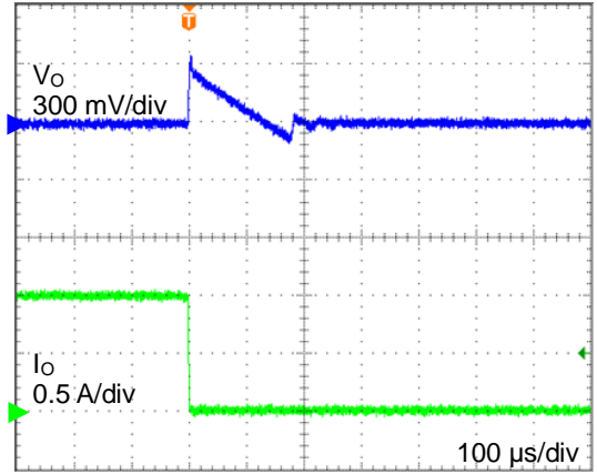
Figure 9. Transient Response (1000 mA \rightarrow 1 mA, T_a = +125\text{ }^\circ\text{C} )
