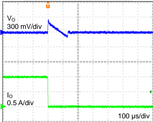
Figure 8. Transient Response (1000 mA \rightarrow 1 mA, T_a = +25\text{ }^\circ\text{C} )
