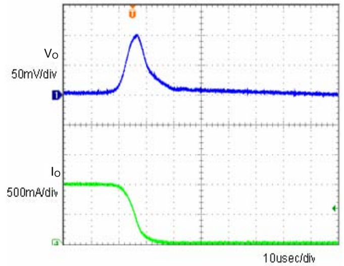
Fig.3 Transient Response (1→0A) Co=1µF
