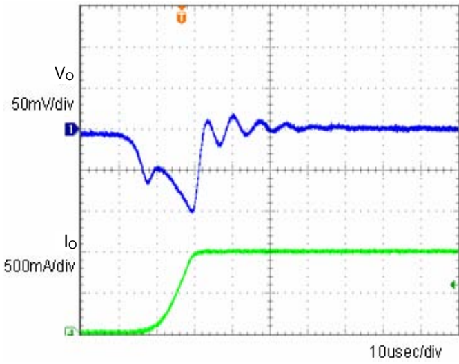
Fig.2 Transient Response (0→1A) Co=1µF
