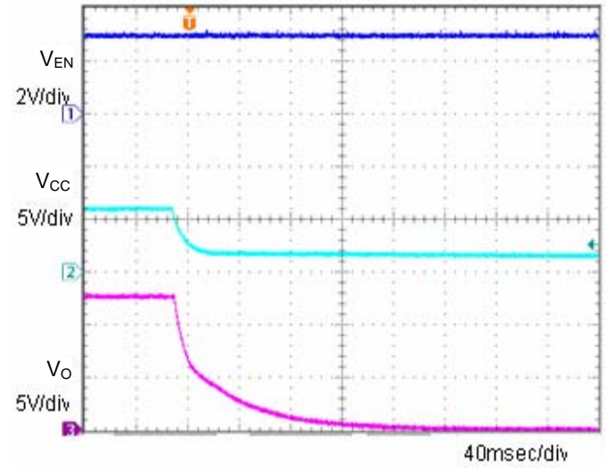
Fig.5 OFF sequence 1 Co=1µF
