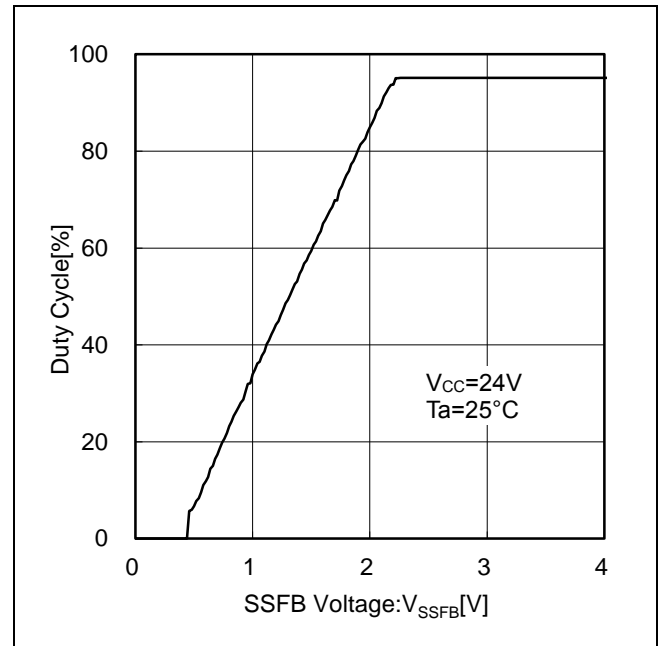
Figure 7. Duty Cycle vs SSFB Voltage
