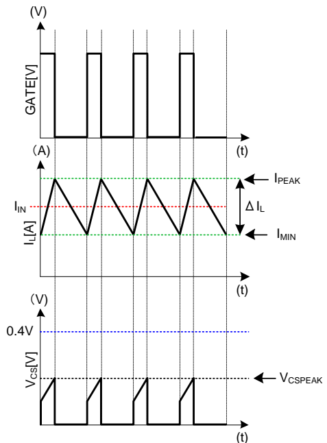
Figure 26. Inductor Current Waveform
