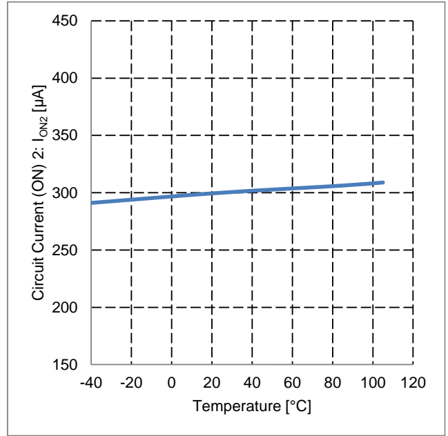
Figure 15. Circuit Current (ON) 2 vs Temperature
