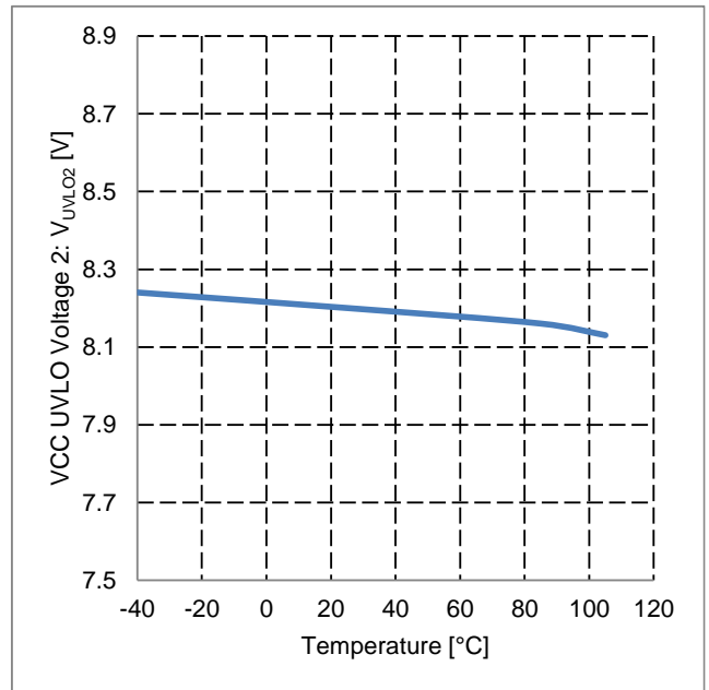
Figure 17. VCC UVLO Voltage 2 vs Temperature
