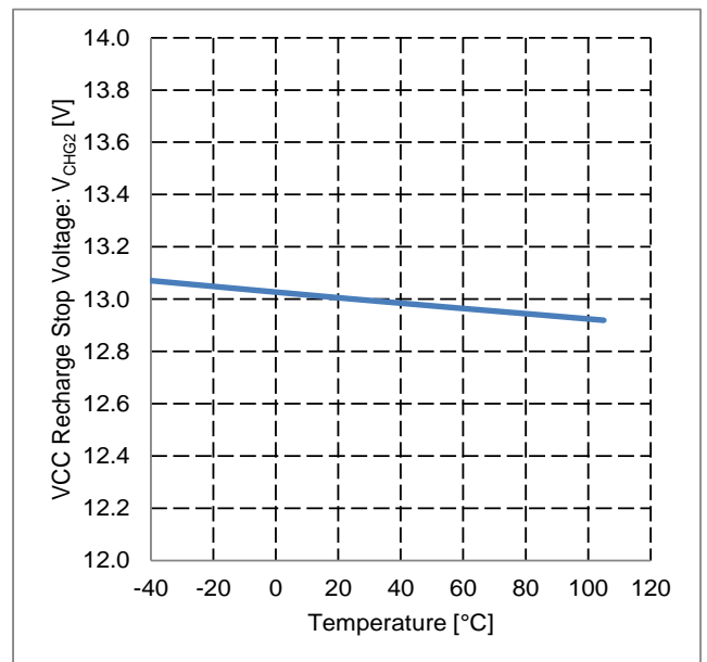
Figure 21. VCC Recharge Stop Voltage vs Temperature
