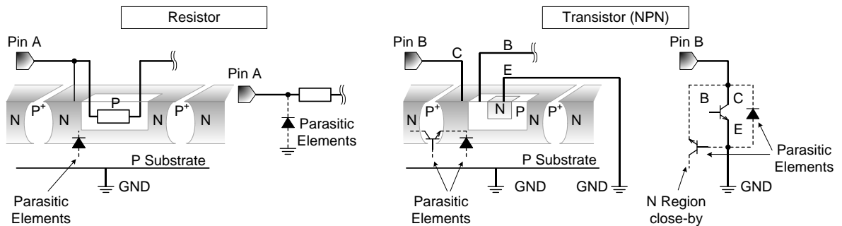
Figure 41. Example of IC Structure
