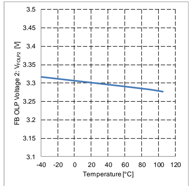
Figure 31. FB OLP Voltage 2 vs Temperature
