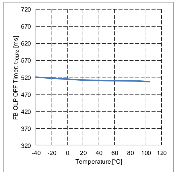
Figure 33. FB OLP OFF Timer vs Temperature
