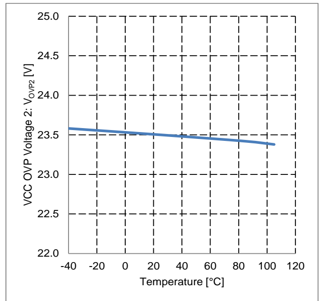
Figure 19. VCC OVP Voltage 2 vs Temperature
