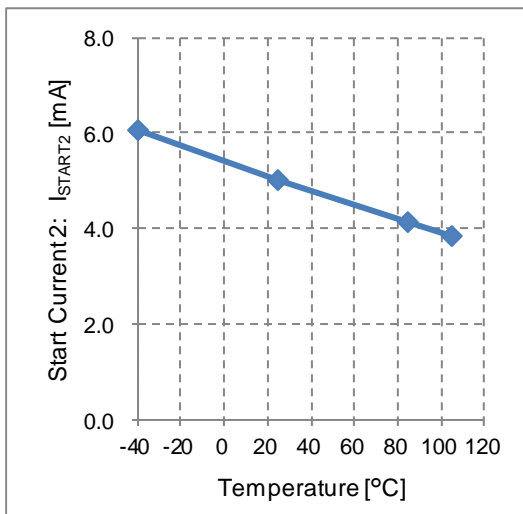
Figure 37. Start Current 2 vs Temperature
