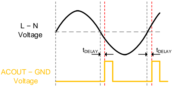
Figure 10. Zero Cross Delay Time (BM1Z003FJ)
