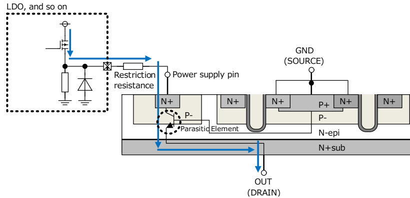
Figure 32. Negative Current Path (when the power supply pin is High)
