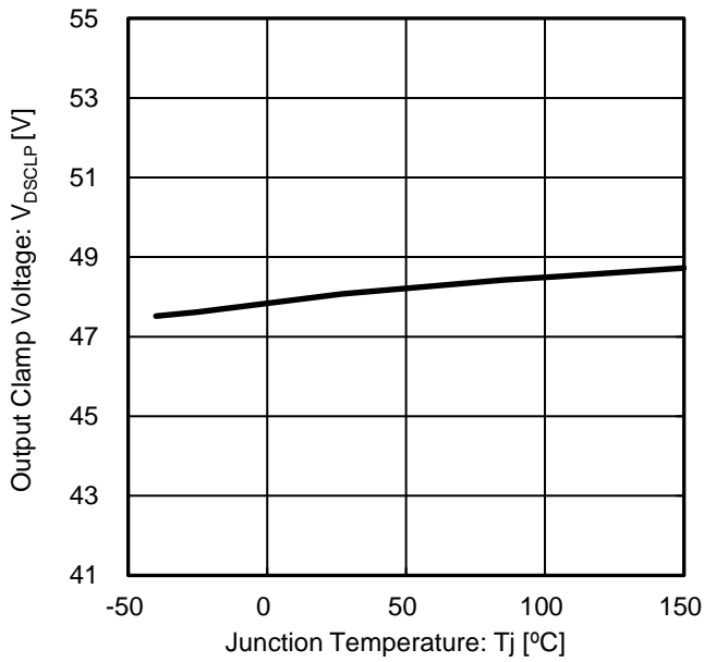
Figure 19. Output Clamp Voltage vs Junction Temperature
