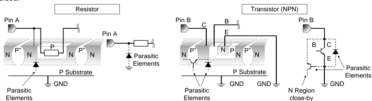
Figure 62. Example of IC Structure
