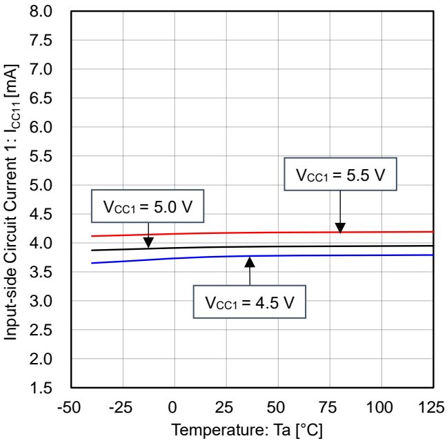
Figure 2. Input-side Circuit Current 1 vs Temperature
