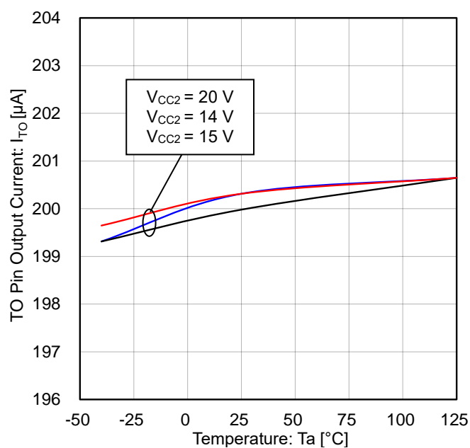
Figure 30. TO Pin Output Current vs Temperature
