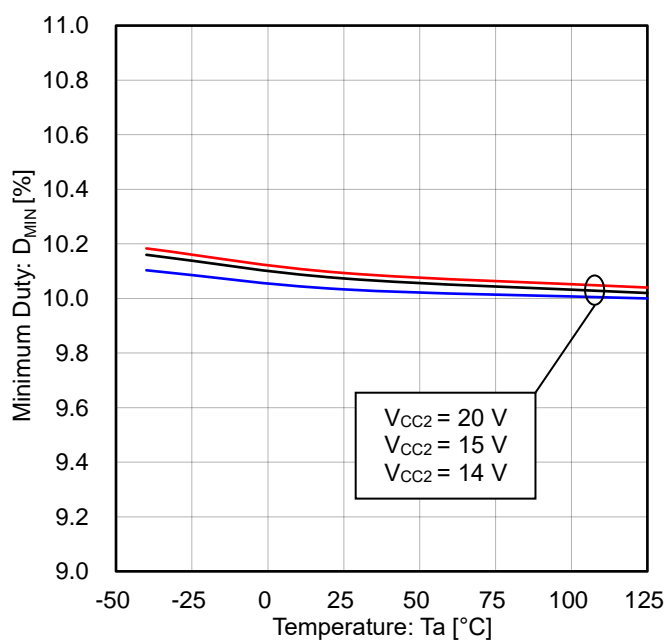
Figure 32. Minimum Duty vs Temperature
