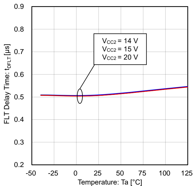
Figure 50. FLT Delay Time vs Temperature
