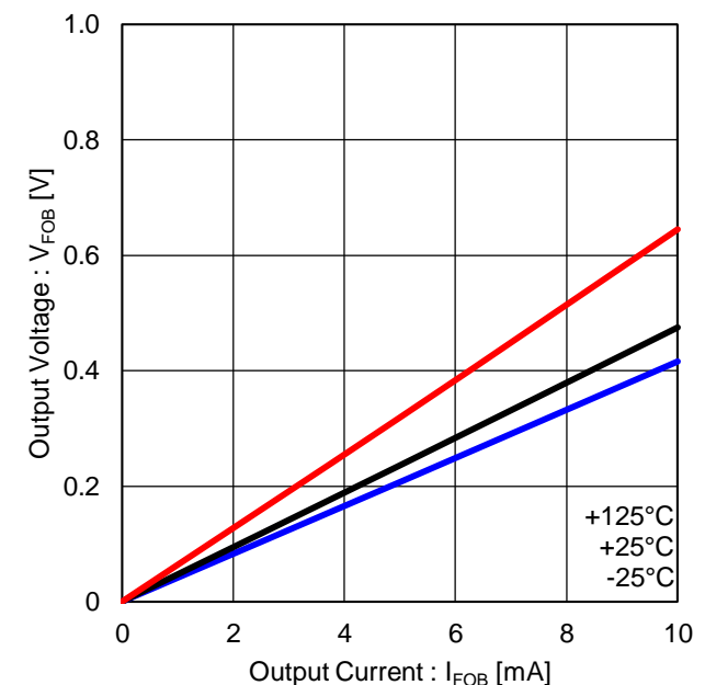
Figure 25. Fault Output ON Resistance
