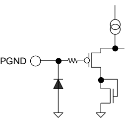
Figure 41. PGND
