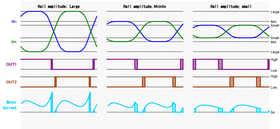
Figure 45. Relation between hall signal amplitude and output wave
