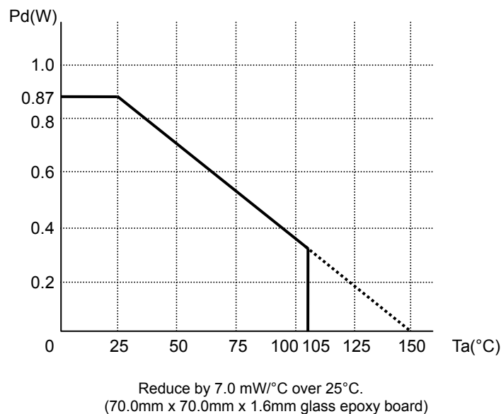
Figure 53. Thermal Derating Curve
