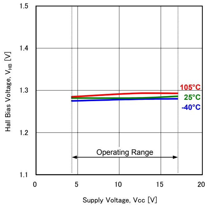
Figure 18. Hall Bias Voltage vs Supply Voltage
