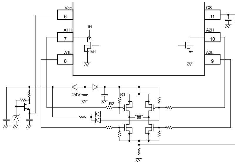
Figure 47. 24V application
