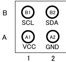
Figure 3. Pin Configuration (BOTTOM VIEW)
