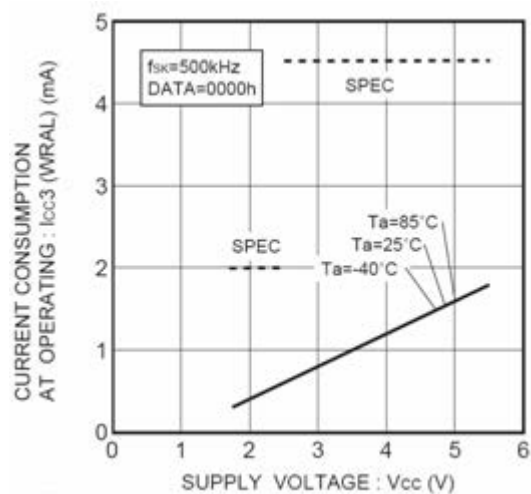
Figure 17. Consumption current at WRAL action ICC3 (WRAL, f_{SK}=500\text{kHz} )
