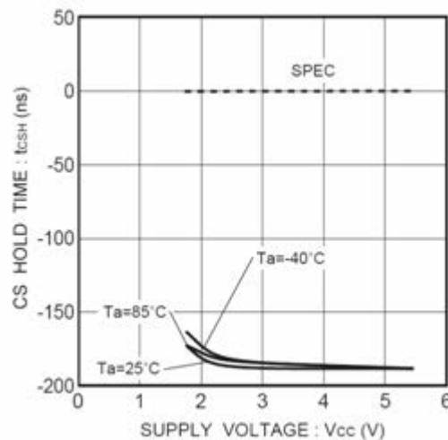
Figure 23. CS hold time tCSH
