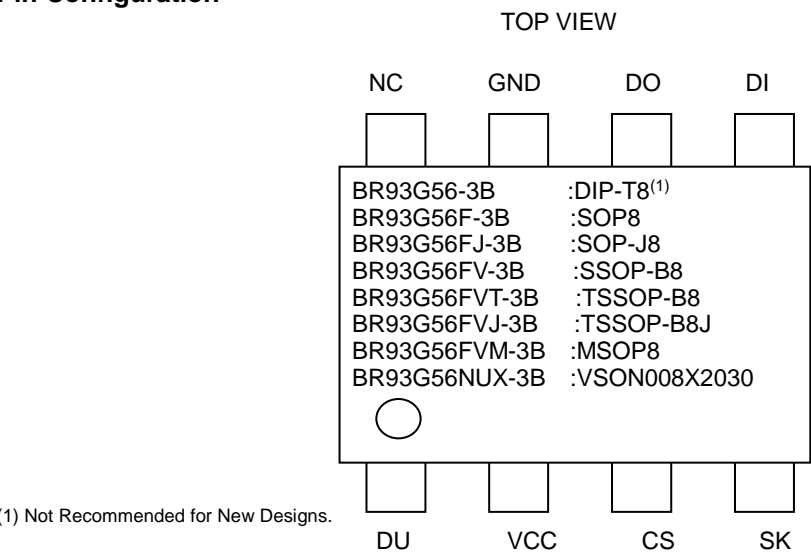
Figure 3. Pin Configuration
