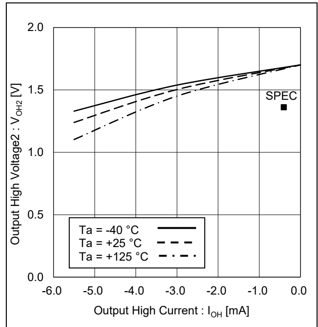
Figure 12. Output High Voltage2 vs Output High Current ( V_{CC} = 1.7 \text{ V} )
