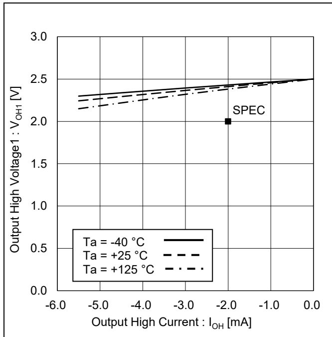
Figure 11. Output High Voltage1 vs Output High Current ( V_{CC} = 2.5 \text{ V} )
