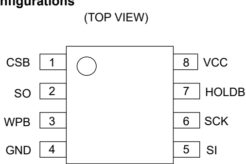
Figure 3-(a). Pin Configuration (SOP8, SOP-J8, TSSOP-B8, MSOP8)
