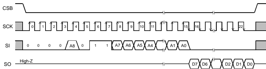
Figure 37. Read command
