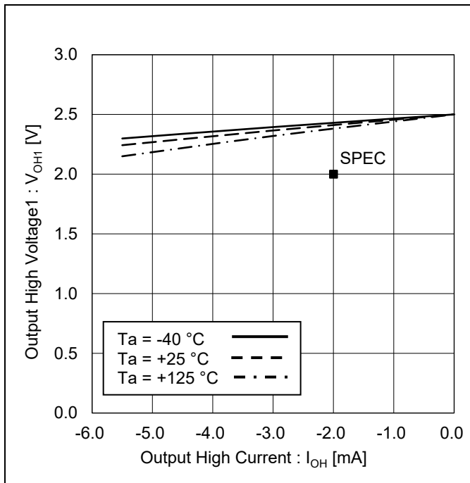
Figure 11. Output High Voltage1 vs Output High Current ( V_{CC} = 2.5\text{ V} )
