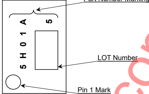
TSSOP-B8 (TOP VIEW)
