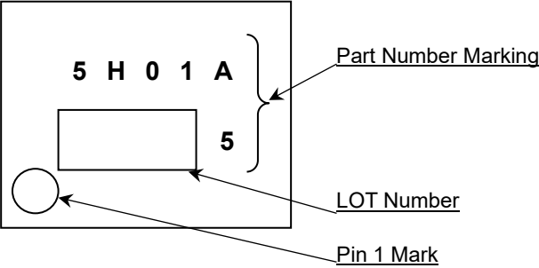
SOP8 (TOP VIEW)
