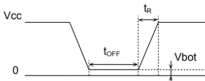
Figure 59. Rise waveform
