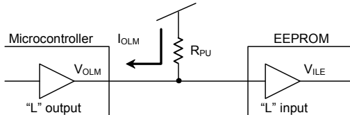
Figure 48. Pull up resistance
