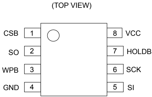
Figure 3-(a). Pin Configuration (SOP-J8, TSSOP-B8, MSOP8)
