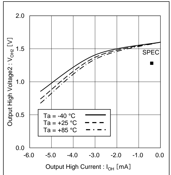
Figure 12. Output High Voltage2 vs Output High Current ( V_{CC} = 1.6\text{ V} )
