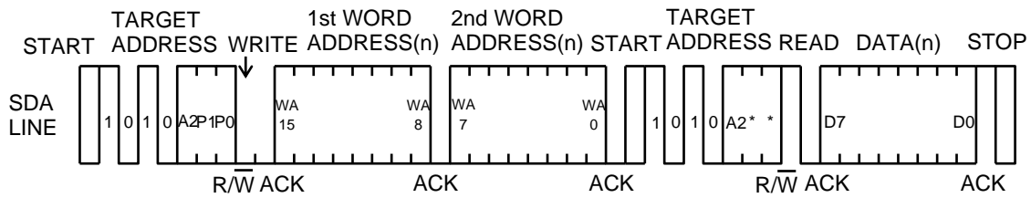
Figure 44. Random Read
