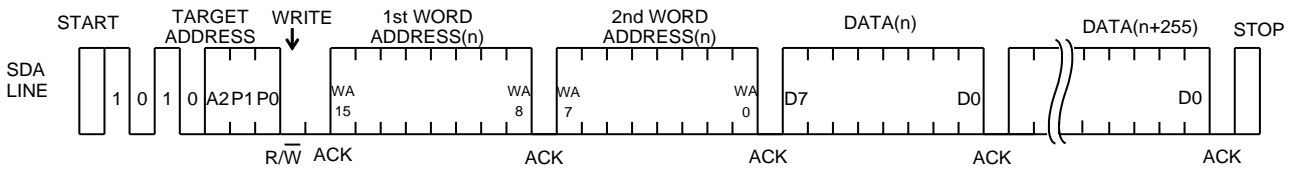
Figure 42. Page Write
