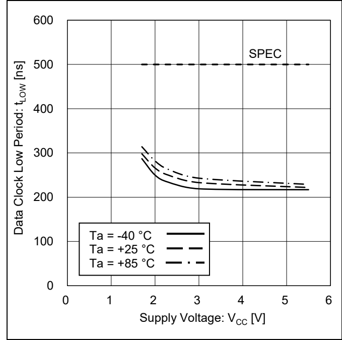
Figure 18. Data Clock Low Period vs Supply Voltage
