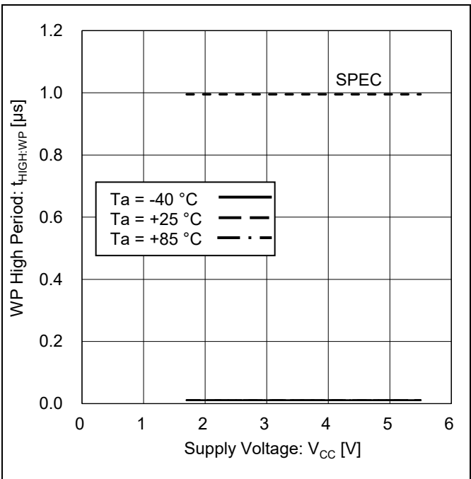
Figure 39. WP High Period vs Supply Voltage
