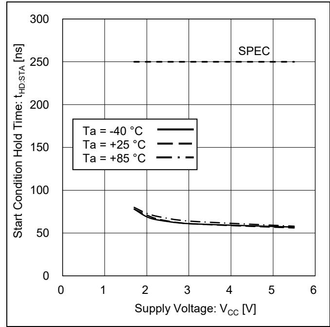
Figure 20. Start Condition Hold Time vs Supply Voltage
